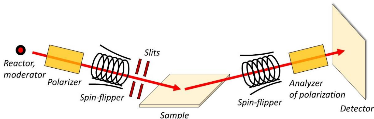
Fig.1. Layout of a polarized neutron reflectometer
