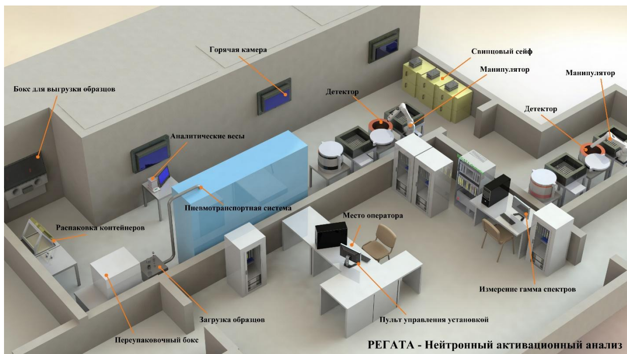
The scheme of the installation
