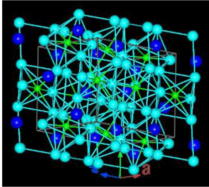
Figure 1b Unit cell of LaMnO_3 (FullProf)
