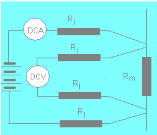
Figure 6 The simplified schema electrical measurements (environment and computer connections are not presented)
