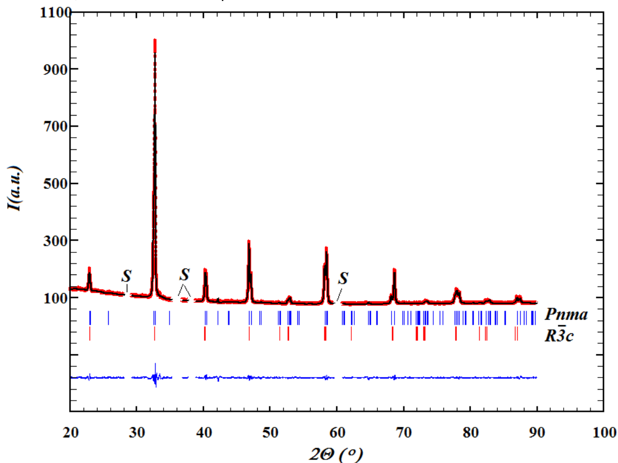
Figure 3. Observed (black) and calculated (red) XRD diffractograms of \text{La}_{0.54}\text{Ho}_{0.11}\text{Sr}_{0.35}\text{Mn}_{0.90}\text{Cr}_{0.10}\text{O}_3 using FullProf software; bottom (blue) – the difference between the calculated and observed diffractograms. S - foreign phase
