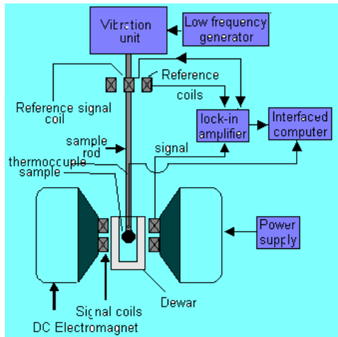
Figure 4 The simplified schema of vibrating sample magnetometer
