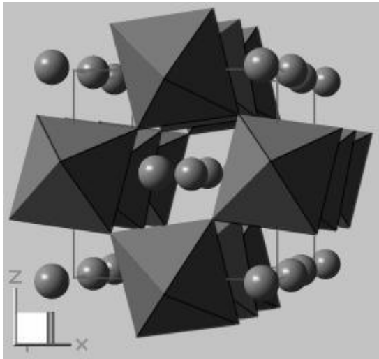
Figure 1a BO_6 octahedra chains orthorhombic structure of LHMCO manganite
