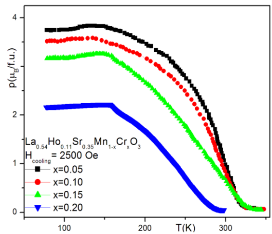
Figure 5 Variation of specific magnetization with the Cr concentration manganites; H_{cool} = H_{measurement} = 2500 Oe
