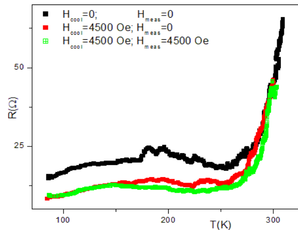
Figure 7 Variation of the resistance with temperature and applied magnetic field for La_{0.54}Ho_{0.11}Sr_{0.35}Mn_{0.95}Cr_{0.05}O_3 .
